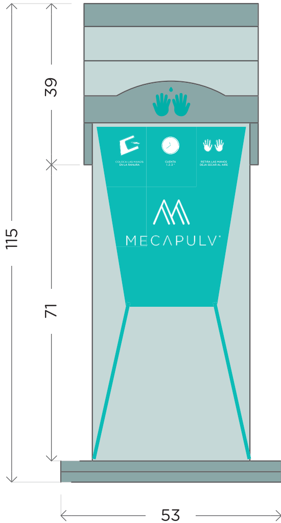
ALZADO PRINCIPAL
